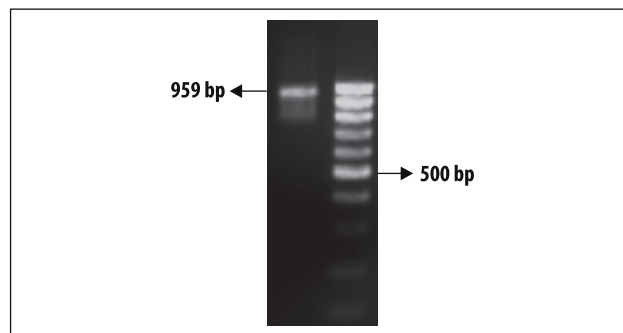
Amplification of 959 bp traA gene from R. equi plasmid DNA. M: 100 bp DNA ladder
