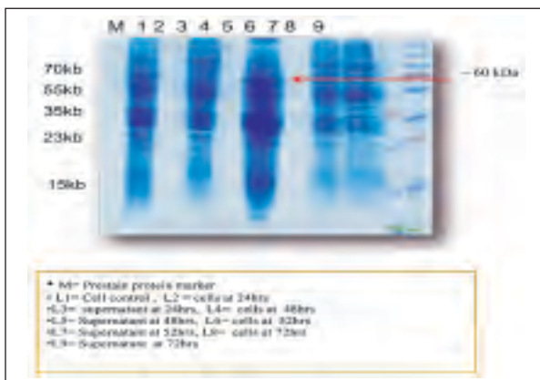
Fig. 7. Expression of rgM in sf9 cells
