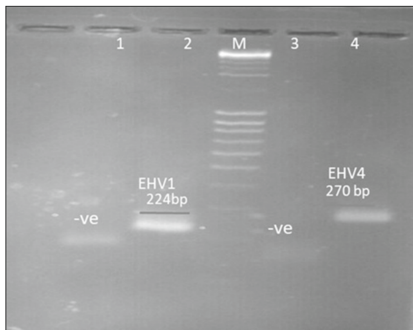
Fig. Isothermal RPA amplification of EHV1 & 4. L1 : -ve control, L2 : Amplification of EHV1 (224 bp), M : 100 bp DNA ladder, L3 : -ve control, L4 : Amplification of EHV4 (270 bp)
